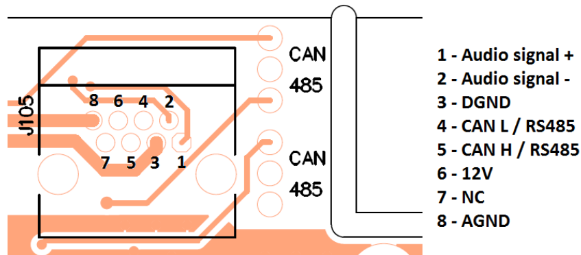
eMPAGE RJ45 connector pinout diagram, CAN bus mode
