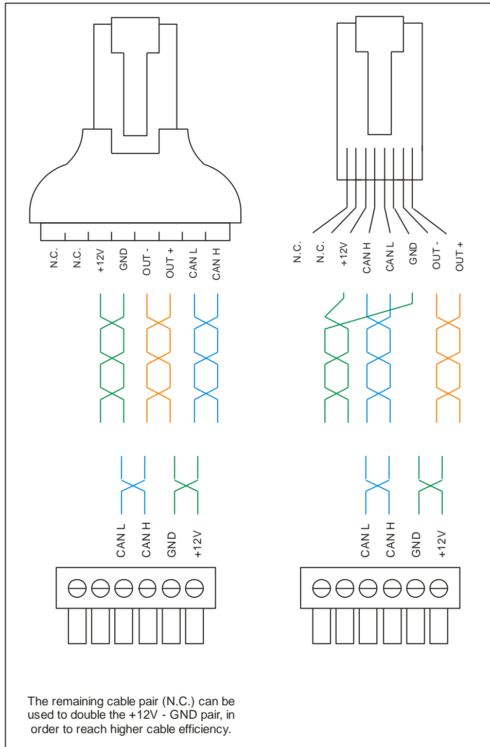
Both possibilities of connection between eMPAGE and the REMOTE ports in MIMO matrices. Left- with the RJ45 to screw terminals adapter / Right – without it, when no daisy-chained units share the same REMOTE line
